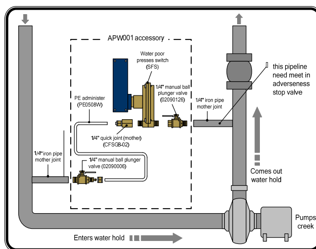
Pictures 2 : SFP and SFS install sketch
