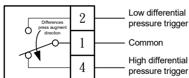
Pictures 1 : SFP and SFS wiring
